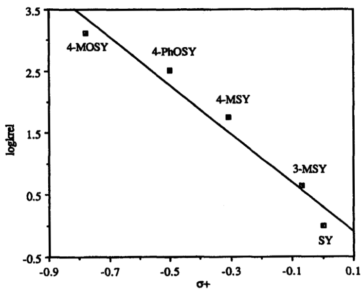
Figure 6. Hammett-Brown plot for the electrochemically induced cycloadditions of substituted trans - \beta -methylstyrenes to 2,3-dimethyl-1,3-butadiene in acetonitrile at +1.5 V vs SCE. \rho = -3.94 ; r^2 = 0.958
