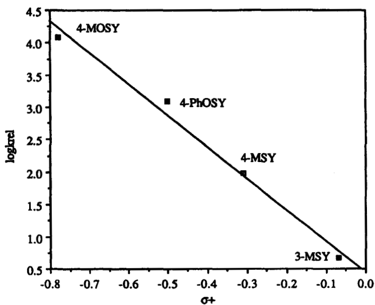
Figure 5. Hammett-Brown plot for the electrochemically induced cycloadditions of substituted trans - \beta -methylstyrenes to 2,3-dimethyl-1,3-butadiene in acetonitrile at +1.1 V vs SCE. \rho = -4.85 ; r^2 = 0.987
