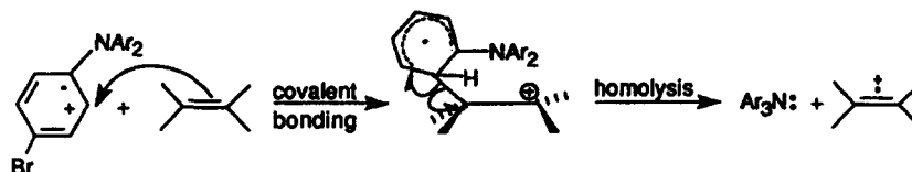
Scheme 1. Outer sphere vs inner sphere electron transfer
