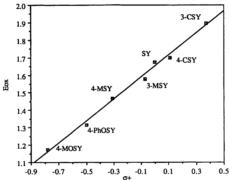
Figure 3. Plot of the oxidation potentials ( E_{ox} ) of substituted trans - \beta -methylstyrenes vs \sigma^+ . Slope = 0.628; r^2 = 0.992
