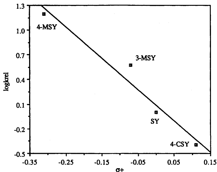
Figure 4. Hammett-Brown for the Diels-Alder cycloadditions of substituted trans - \beta -methylstyrenes to 2,3-dimethyl-1,3-butadiene, catalyzed by 5^{+} in dichloromethane at 0^{\circ}\text{C} . \rho = 3.82 ; r^2 = 0.953
