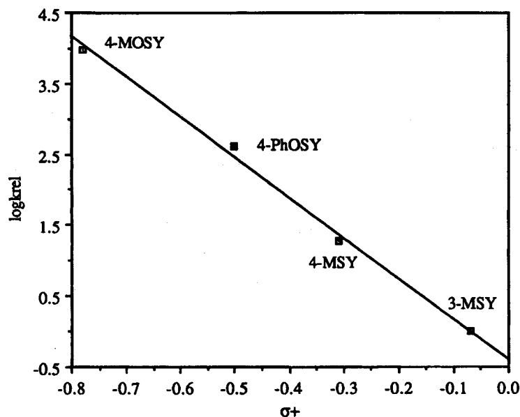
Figure 1. Hammett-Brown plot for the Diels-Alder cycloadditions of substituted trans - \beta -methylstyrenes to 2,3-dimethyl-1,3-butadiene, catalyzed by 1^{+} in dichloromethane at 0°C. SY = trans - \beta -methylstyrene; MO = methoxy; PhO = phenoxy; M = methyl; \rho = -5.70 ; r^2 = 0.996
