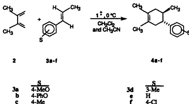
Scheme 3. The Diels-Alder reactions of trans - \beta -methylstyrenes with 2,3-dimethyl-1,3-butadiene, catalyzed by 1^{\dot{+}}
