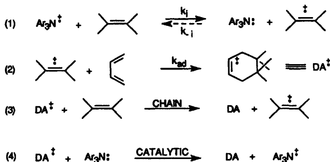
Scheme 1. Outer sphere vs inner sphere electron transfer
