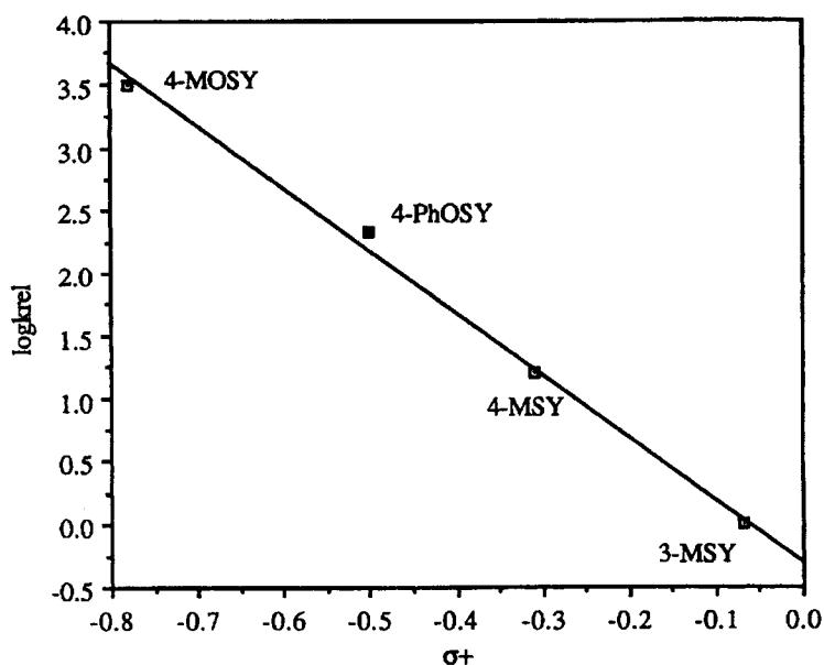
Figure 2. Hammett-Brown plot for the Diels-Alder cycloadditions of substituted trans - \beta -methylstyrenes to 2,3-dimethyl-1,3-butadiene, catalyzed by 1^+ in acetonitrile at 0°C. \rho = -4.99 ; r^2 = 0.995
